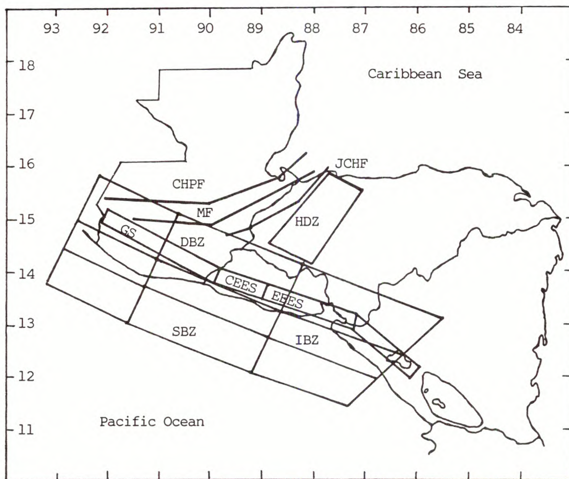
Fig. 6. Seismogenic sources used in hazard study by Alfaro et al. (1990). SBZ-shallow Benioff zone, IBZ-intermediate Benioff zone, DBZ-deep Benioff zone, CHPF-Chixoy-Polochic fault, MF-Motagua fault, JCHF-Jocotan-Chamelecon fault, HDZ-Honduran depression, GS-Guatemalan section of volcanic chain, EEES-eastern El Salvador section of volcanic chain, CEES-central El Salvador section of volcanic chain.
