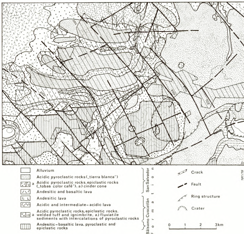
Fig. 2: Geological map of the San Salvador area
